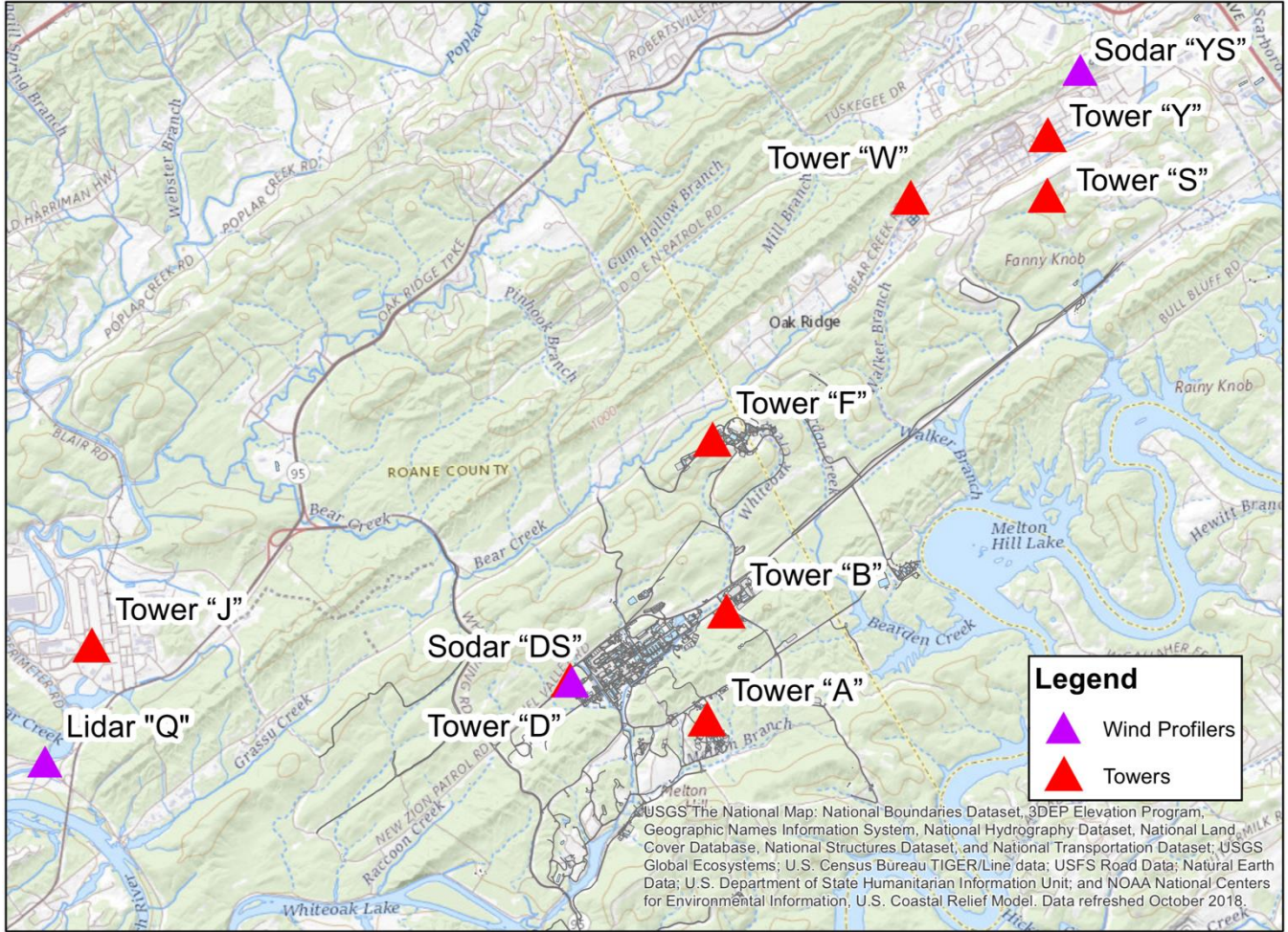
Figure 3-2: Locations of meteorological towers and wind profilers at ETTP, ORNL, and Y-12
