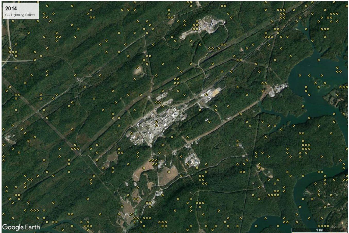
Figure 3-19: Lightning strikes recorded at or near ORNL during 2014
