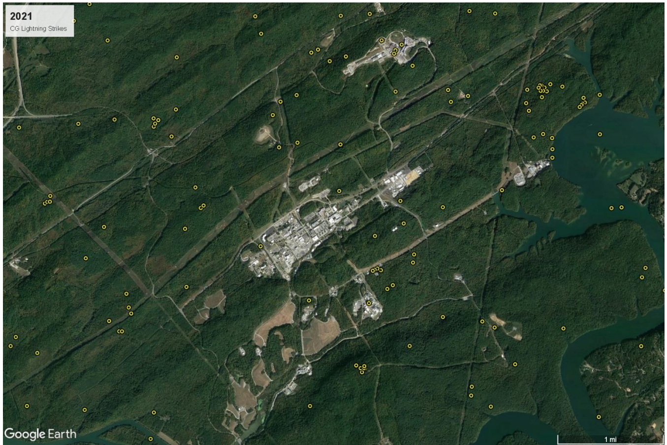
Figure 3-26: Lightning strikes recorded at or near ORNL during 2021
