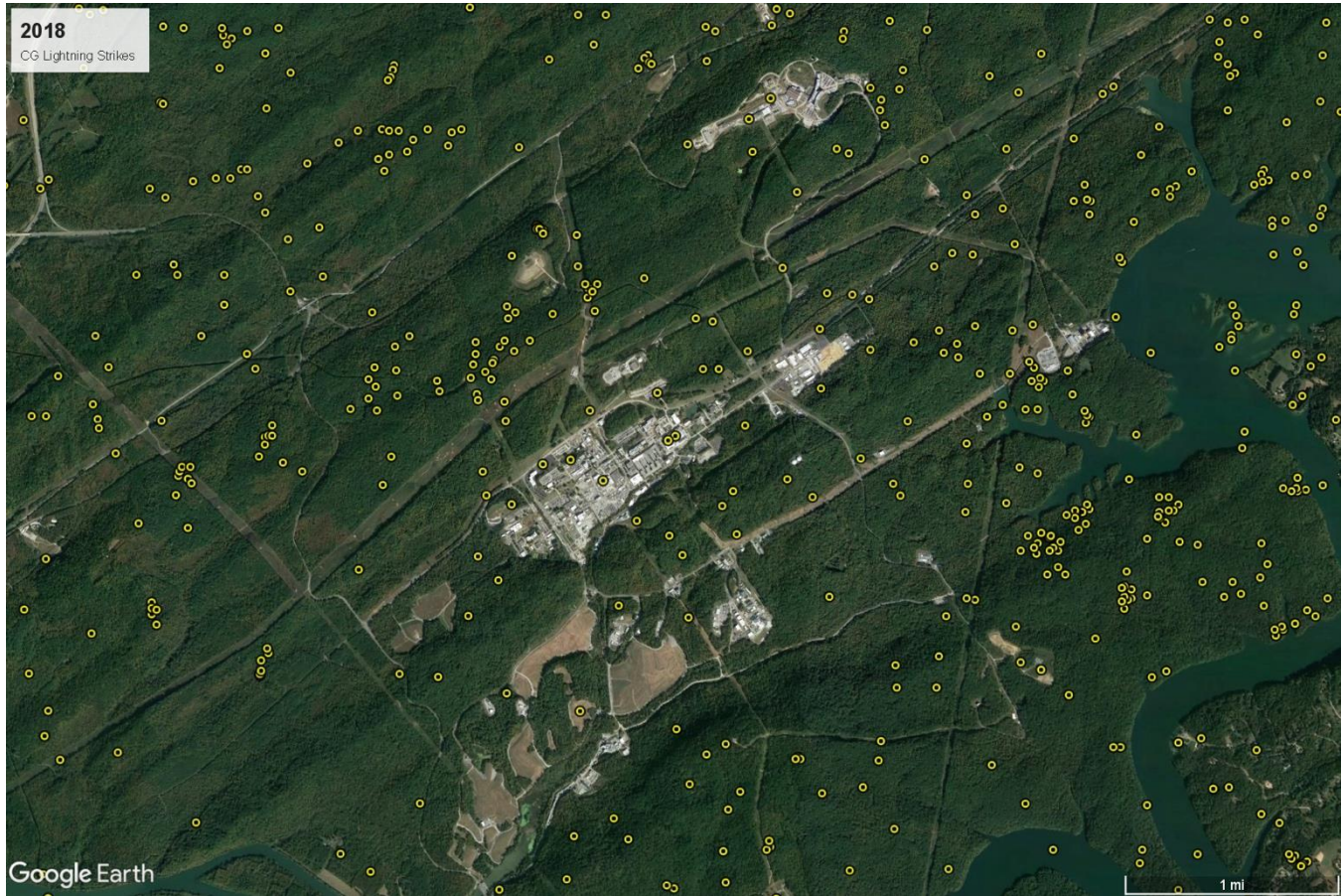
Figure 3-23: Lightning strikes recorded at or near ORNL during 2018
