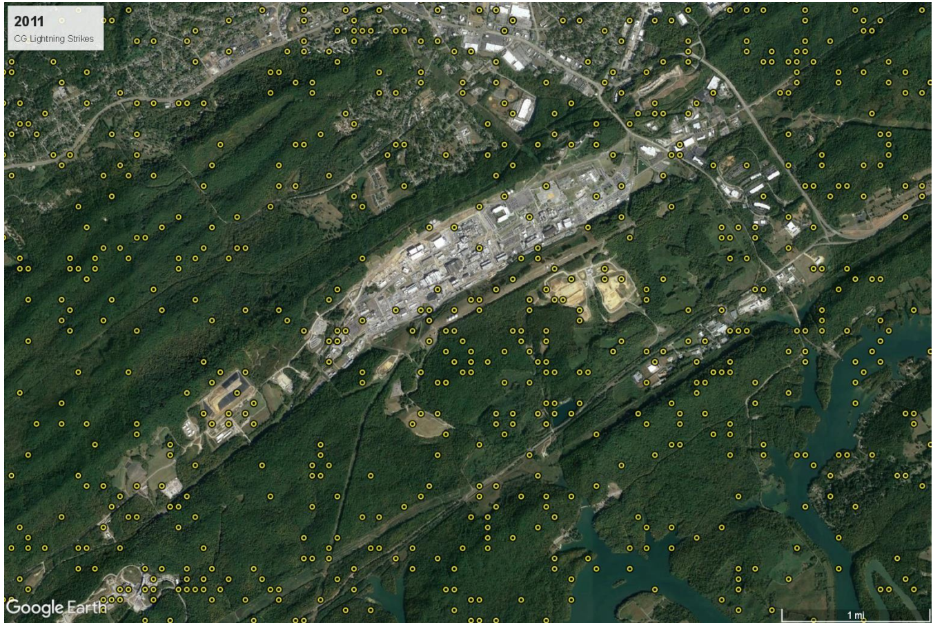
Figure 3-28: Lightning strikes recorded at or near Y-12 during 2011
