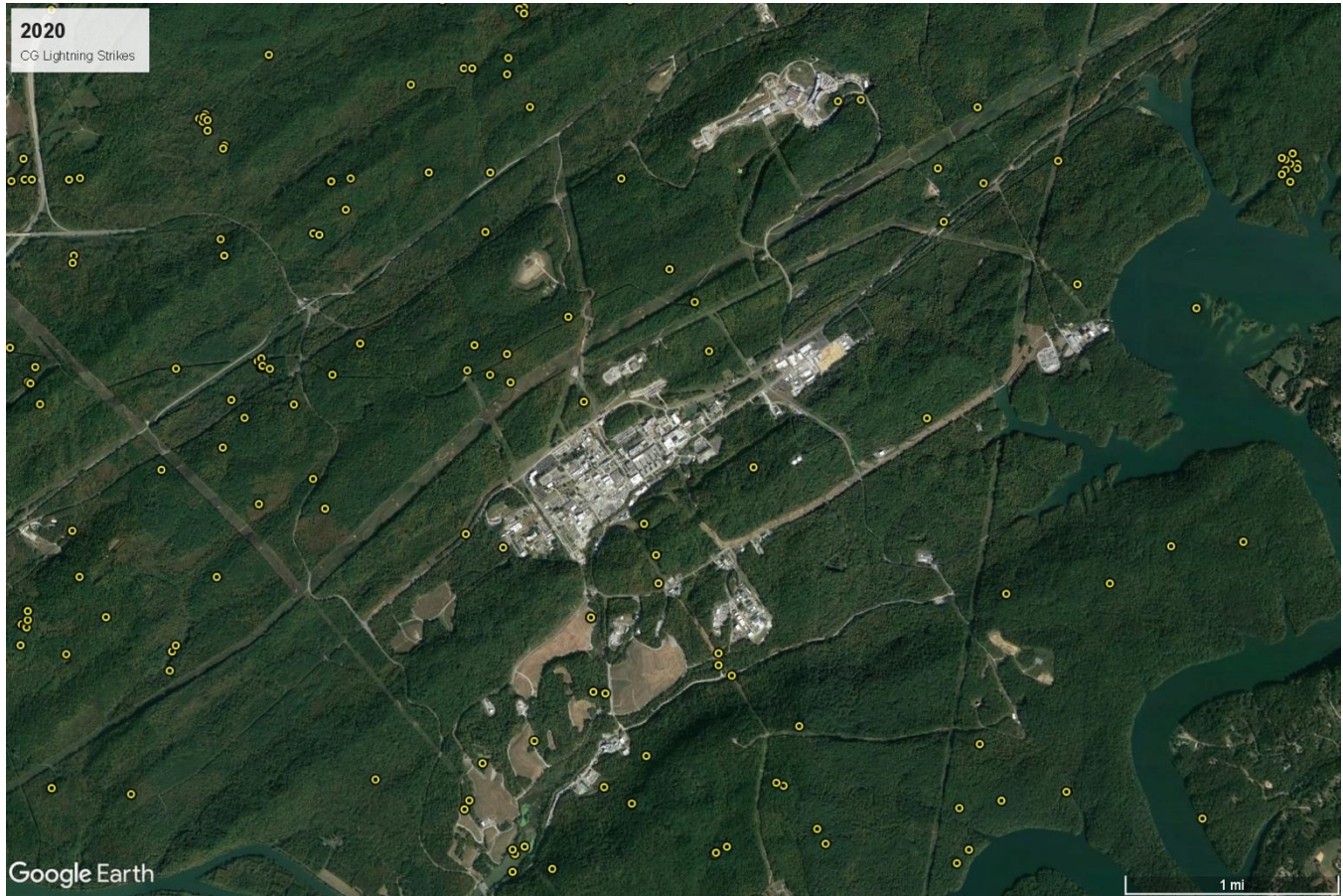
Figure 3-25: Lightning strikes recorded at or near ORNL during 2020
