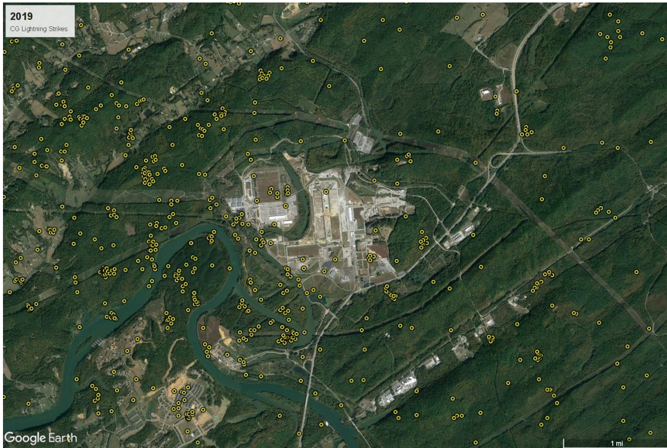
Figure 3-12: Lightning strikes recorded at or near ETPP during 2019
