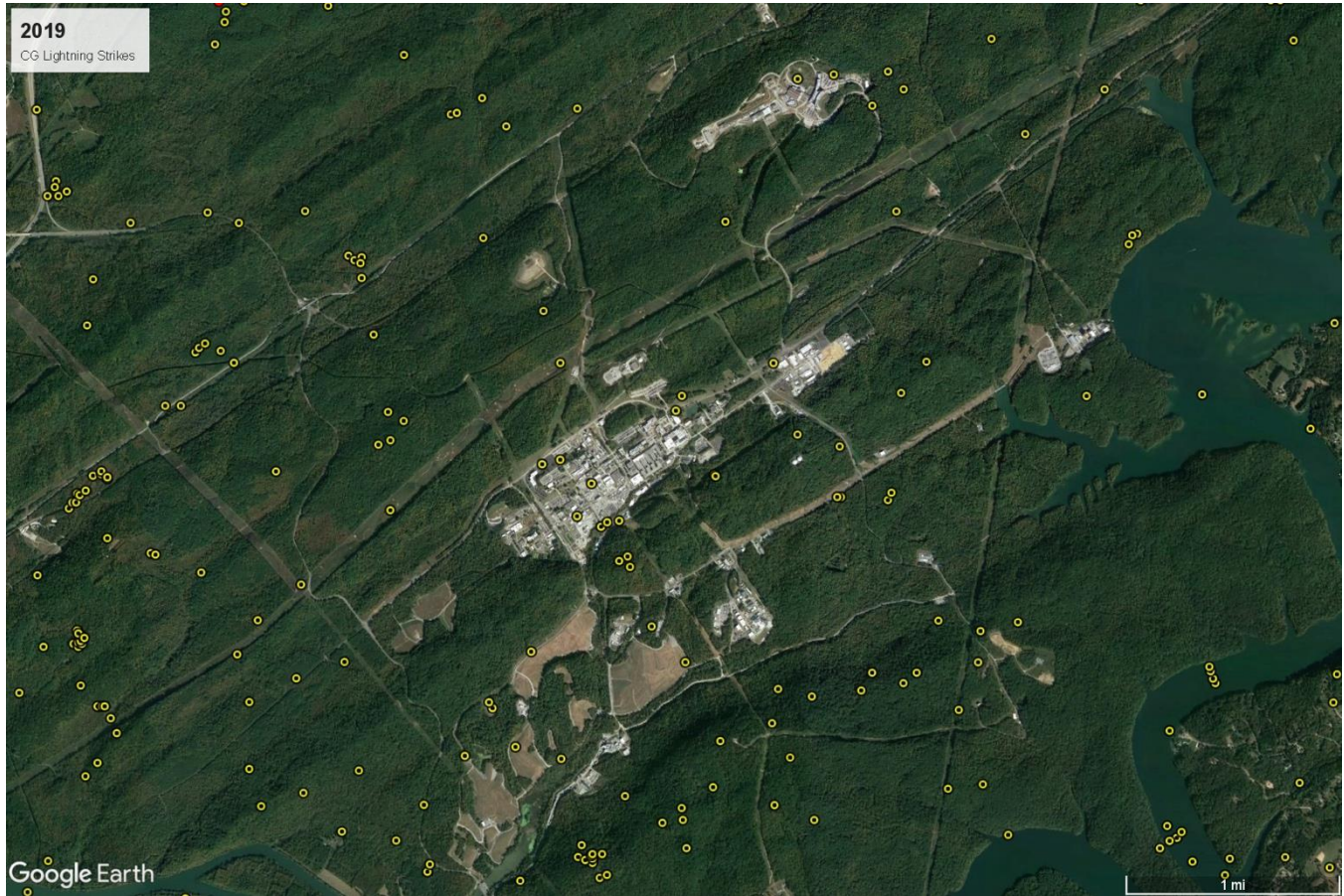
Figure 3-24: Lightning strikes recorded at or near ORNL during 2019
